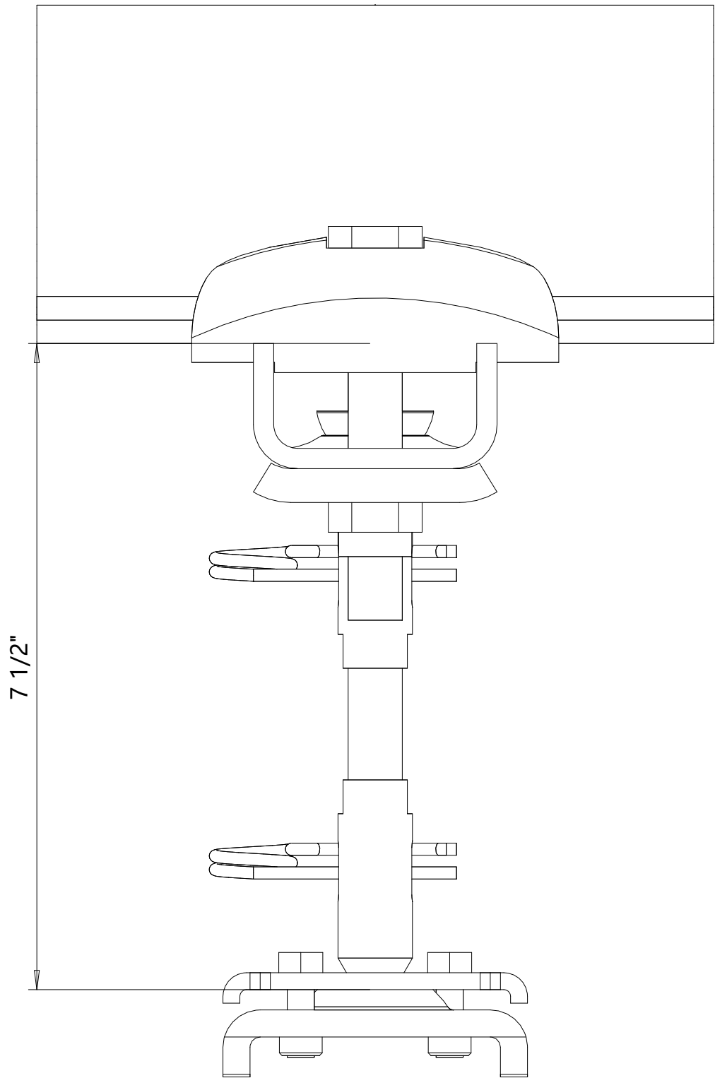
A1 Upper susp. bracket A suits for FLANGE WIDTHS 2 13/16" - 5 1/2"
